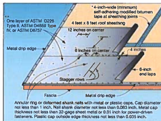
Sealed Roof Deck Option #2
